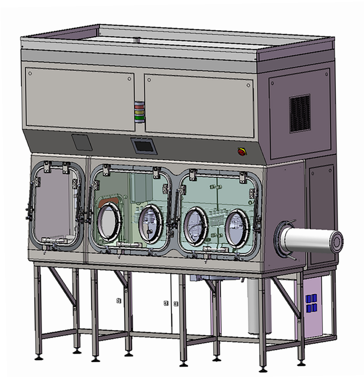
Isolator for product protection | Praha Vaccines a.s. | Czech Republic
